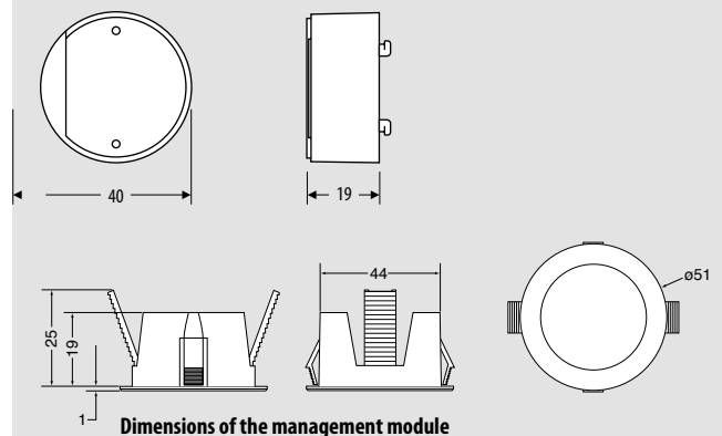
Dimensions of the management module
