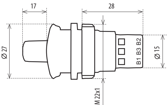
External potentiometer for CRM-2HE, CRM-91HE
