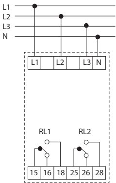
4-wire connection
