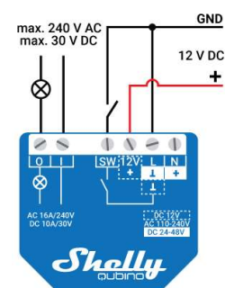
12 V DC
